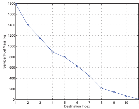
(a) 11 Target Rendezvous Sequence
