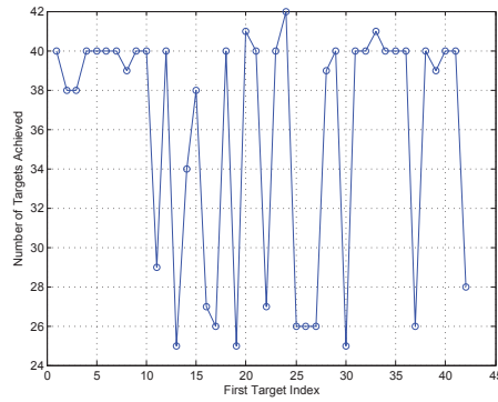
(b) 42 Target Rendezvous Sequence
