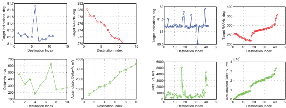
(a) 11 Target Rendezvous Sequence
