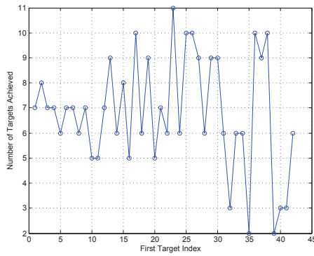
(a) 11 Target Rendezvous Sequence
