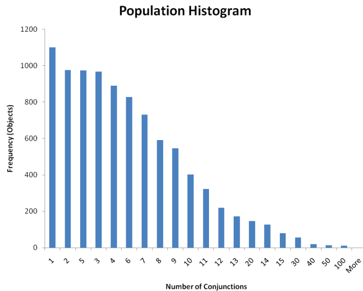
Figure 4. Population Conjunction Histogram for 11 Feb 2009 through 16 Feb 2009
