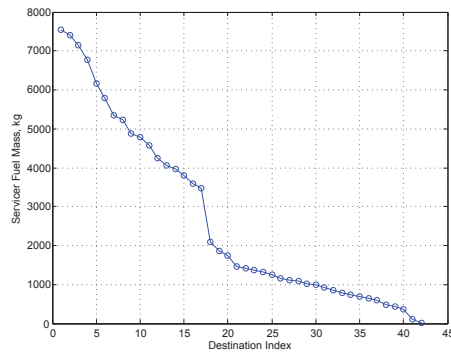
(b) 42 Target Rendezvous Sequence
