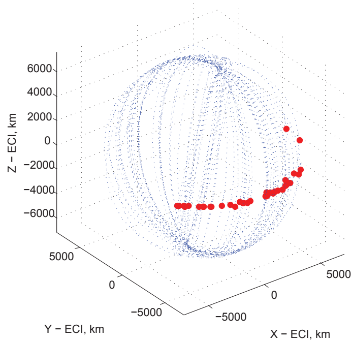
Figure 5. Orbits of the 42 Debris Pieces
